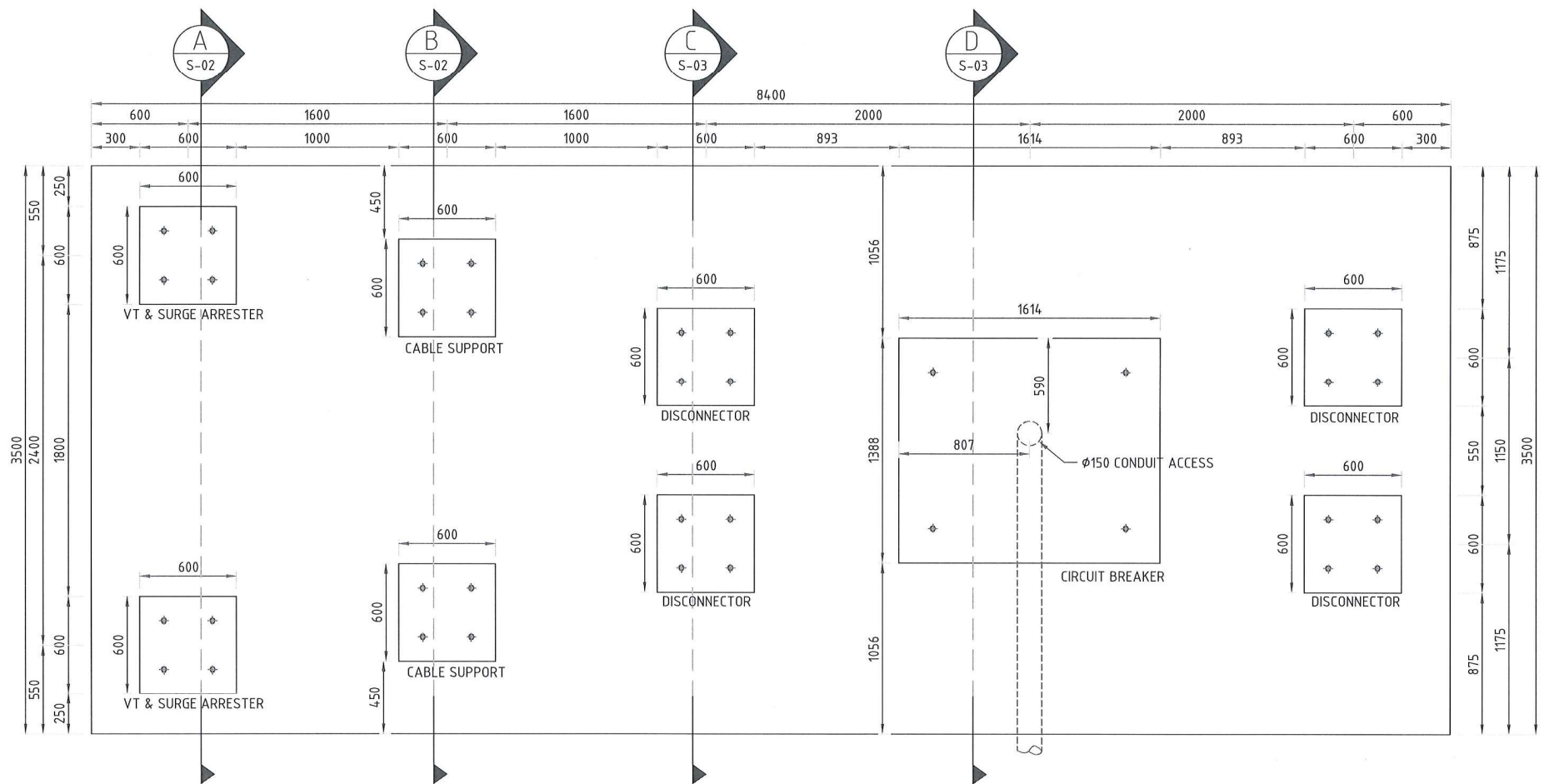
BAY PAD PLAN
