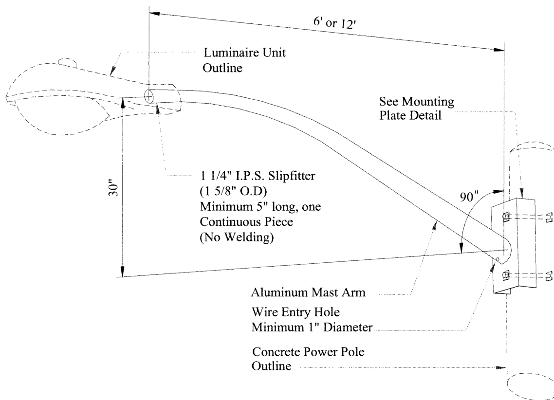
Mast Arm Elevation Detail Figure 1
