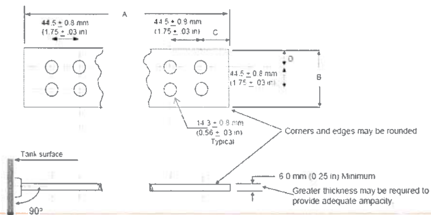
FIGURE 2. Spade Dimensions
