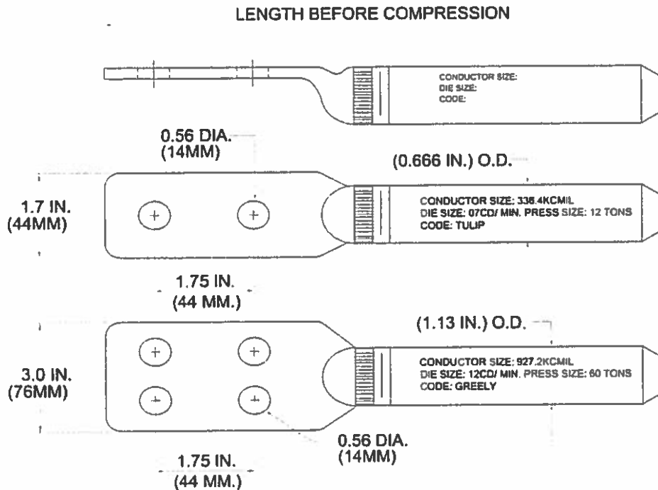
Figure H COMPRESSION JUMPER TERMINAL
