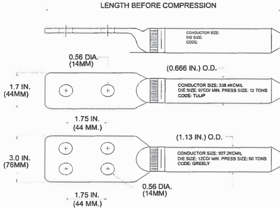
Figure H COMPRESSION JUMPER TERMINAL
