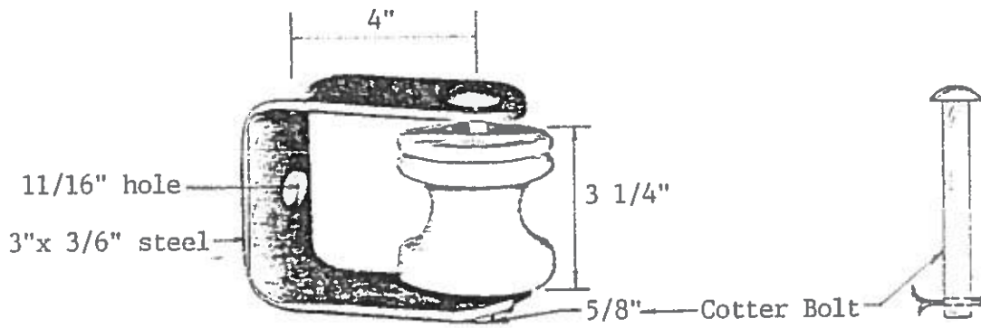
CLEVIS, SECONDARY INDEX No. SSOC0190
