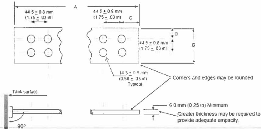
FIGURE 2. Spade Dimensions
