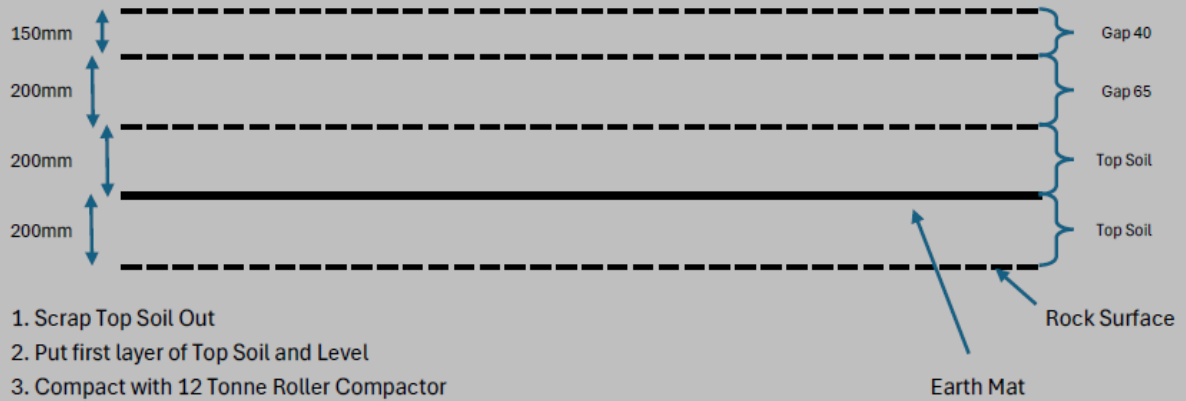
Cawaira Power Station Top Level Platform - Civil Layout
