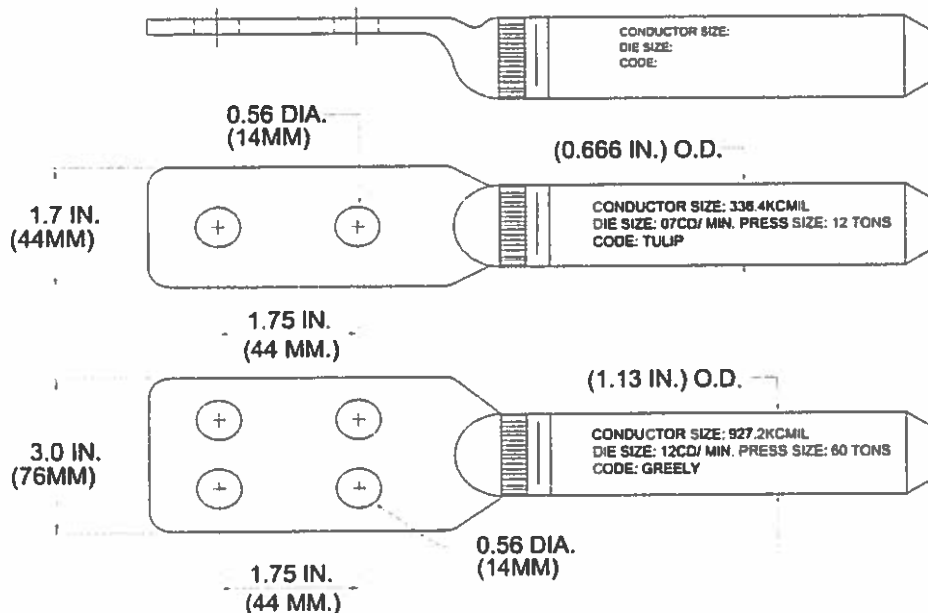
Figure H COMPRESSION JUMPER TERMINAL
