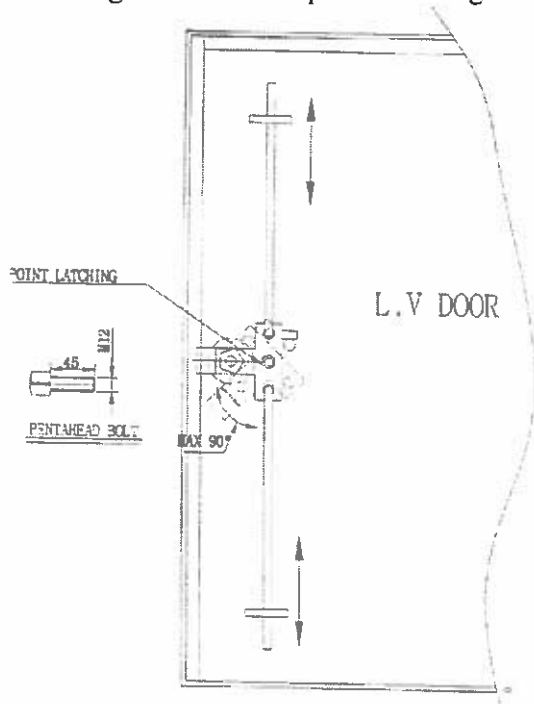
Figure 4 – Three-point latching of Low Voltage Door
