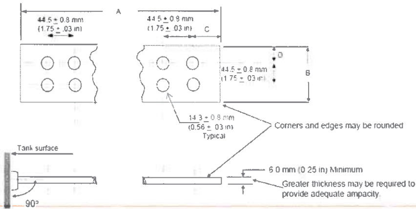
FIGURE 2. Spade Dimensions
