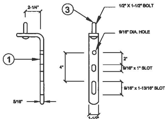
BRACKET DETAIL
