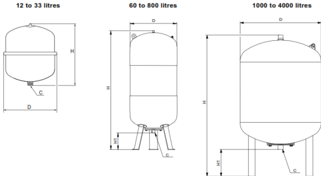
Fig. 5 Dimensional sketches
