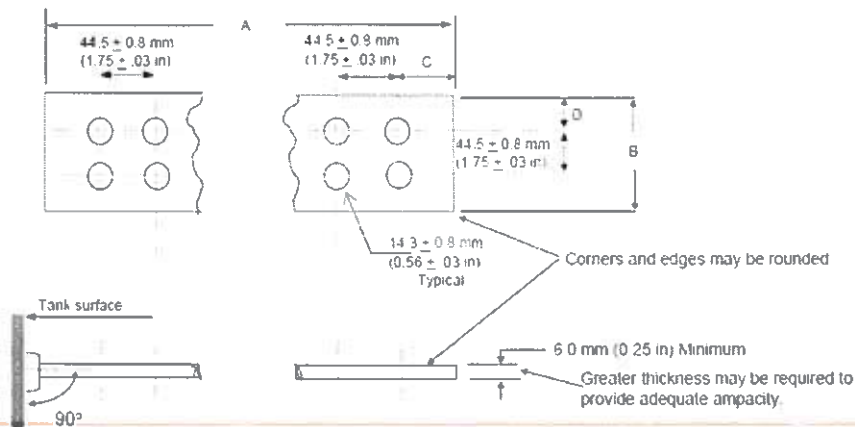
FIGURE 2. Spade Dimensions
