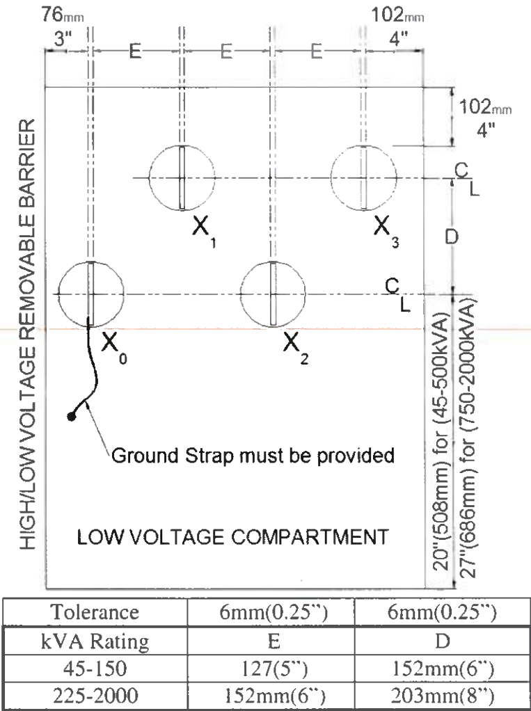
Figure 3 – Staggered Low Voltage terminal minimum dimensions per ANSI C57.12.34-2004 (45kVA added per GPA size requirements)
