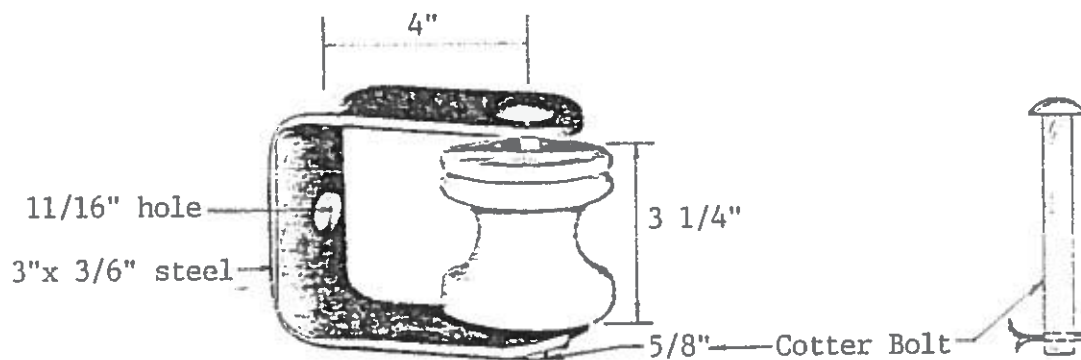
CLEVIS, SECONDARY
