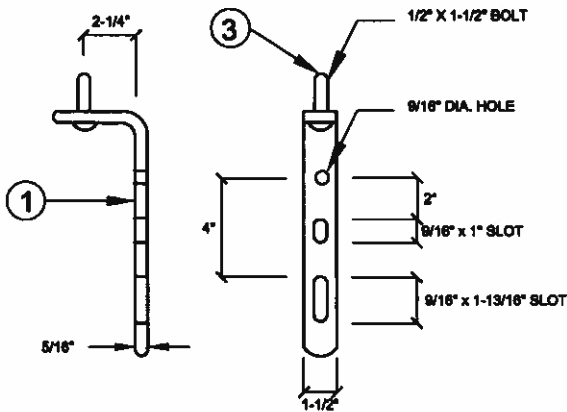
BRACKET DETAIL
