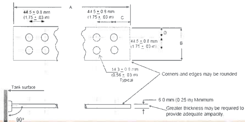
FIGURE 2. Spade Dimensions
