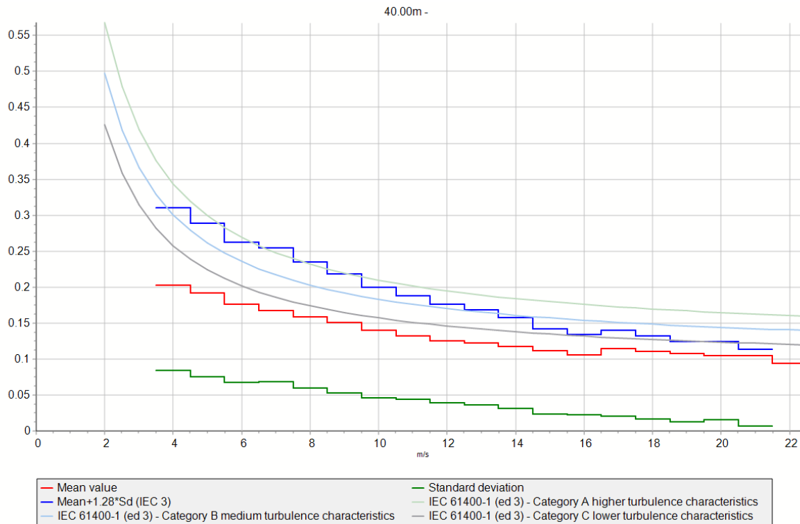
Figure 5: Turbulence at 40 m AGL compared to the IEC curves.
