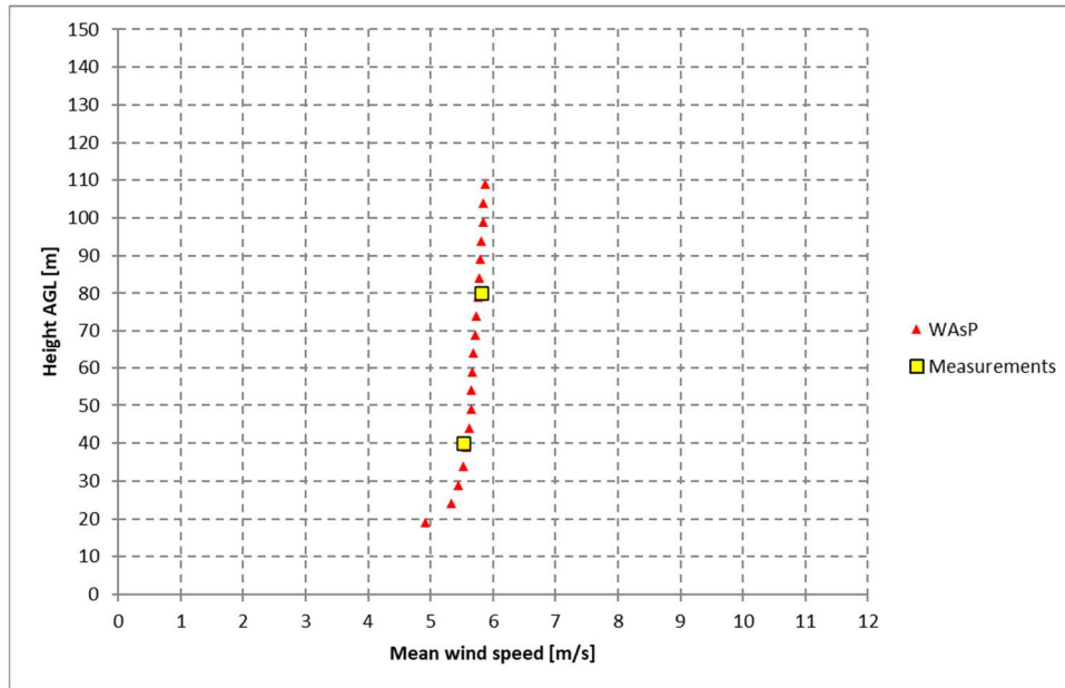
Figure 3: Mean wind speeds measured over the short-term period limited to 3.4 months and vertical wind speed profile calculated by WASP using measurements at 40, 80m AGL
