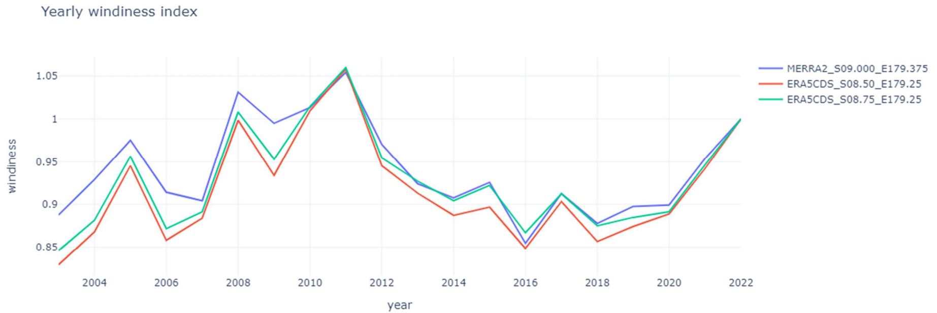
Figure 2: Annual windiness relative to last concurrent year
