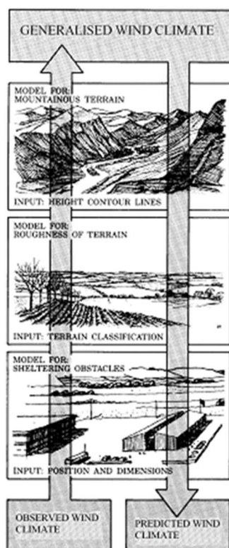
Figure 13: Wind Atlas methodology (Source: wasp.dk)
