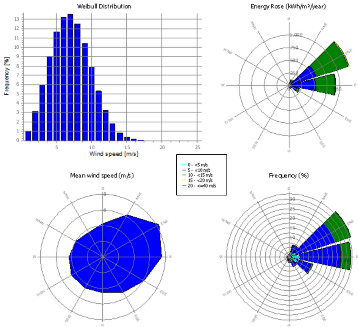
Figure 12: Long-term wind regime at 40.5m AGL at the Lidar
