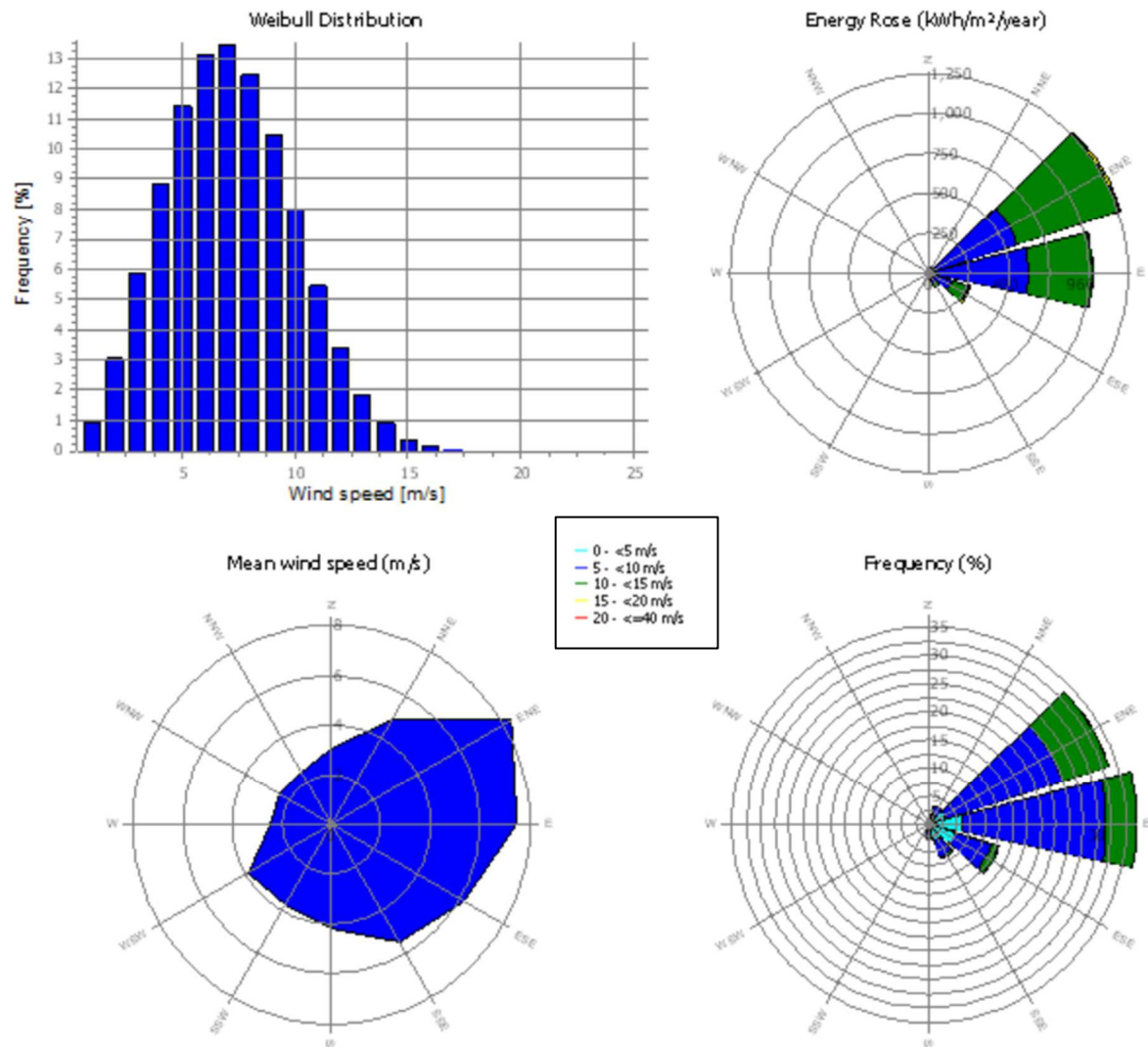
Figure 10: Short-term wind regime at 40.5 m AGL at the Lidar
