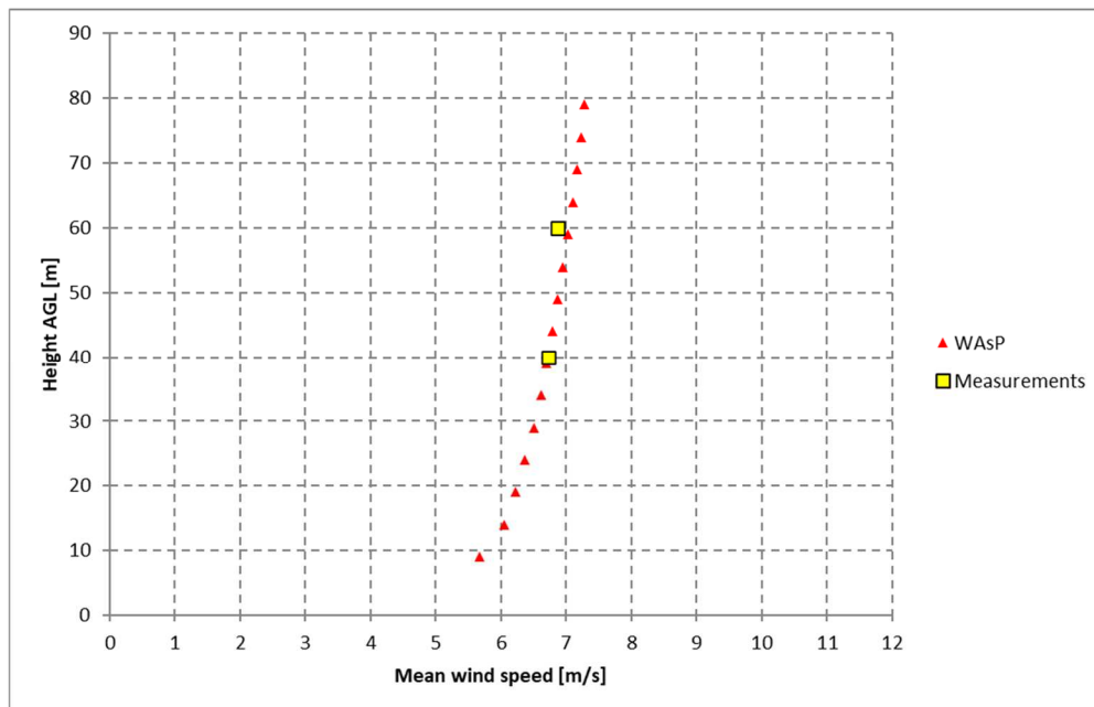
Figure 3: Mean wind speeds measured over the short-term period limited to 12 months and vertical wind speed profile calculated by WAsP using measurements at 40.5,60.5 m AGL
