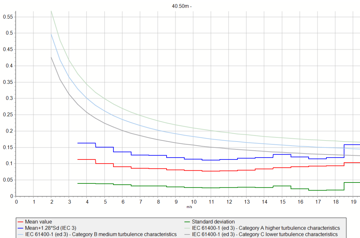
Figure 5: Turbulence at 40.5 m AGL compared to the IEC curves
