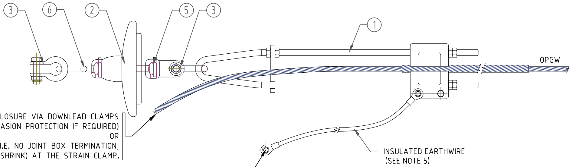
SIDE VIEW
