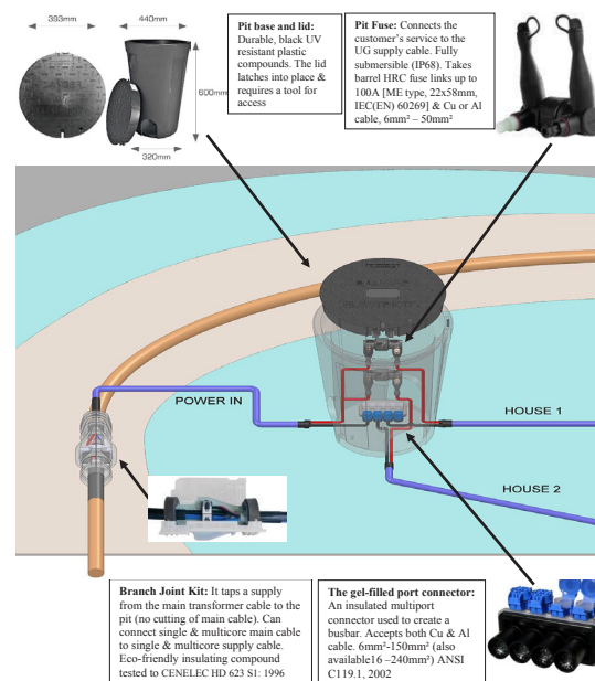
Fig. 9 – Service pit basic layout showing how it works
