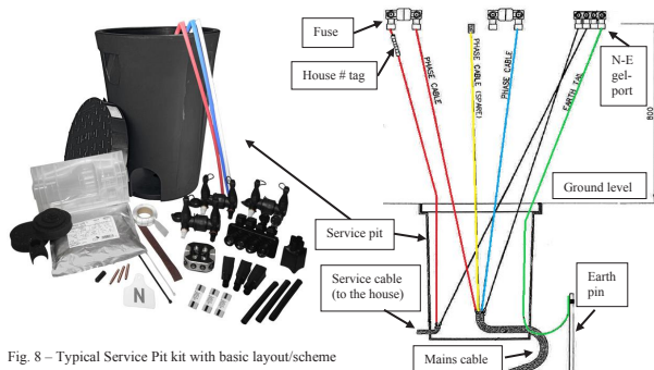
Fig. 8 – Typical Service Pit kit with basic layout/scheme
