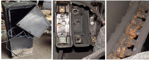
Fig. 2. Burnt plastic service pillar and its internals. Root cause - increased contact resistance and overheating of fuse contact; condensation and corrosion of contacts, including on Neutral-Earth bar
