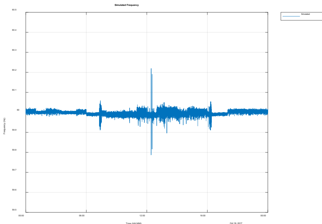
Figure 3-62 Simulated frequency on weekday with current installed PV
