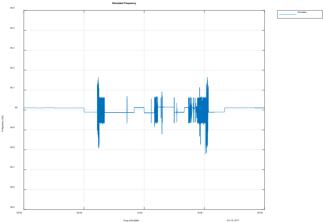
Figure 3-65 Case 21 - Simulated frequency on weekday with 2.3 MW PV and 0.5 MW battery on primary frequency control.
