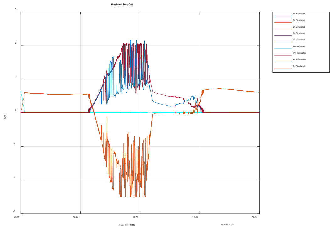
Figure 3-59 Simulated generator outputs for weekday when 2.5 MW / 13 MWh battery provides both primary frequency control and AGC with 4.3 MW of PV.
