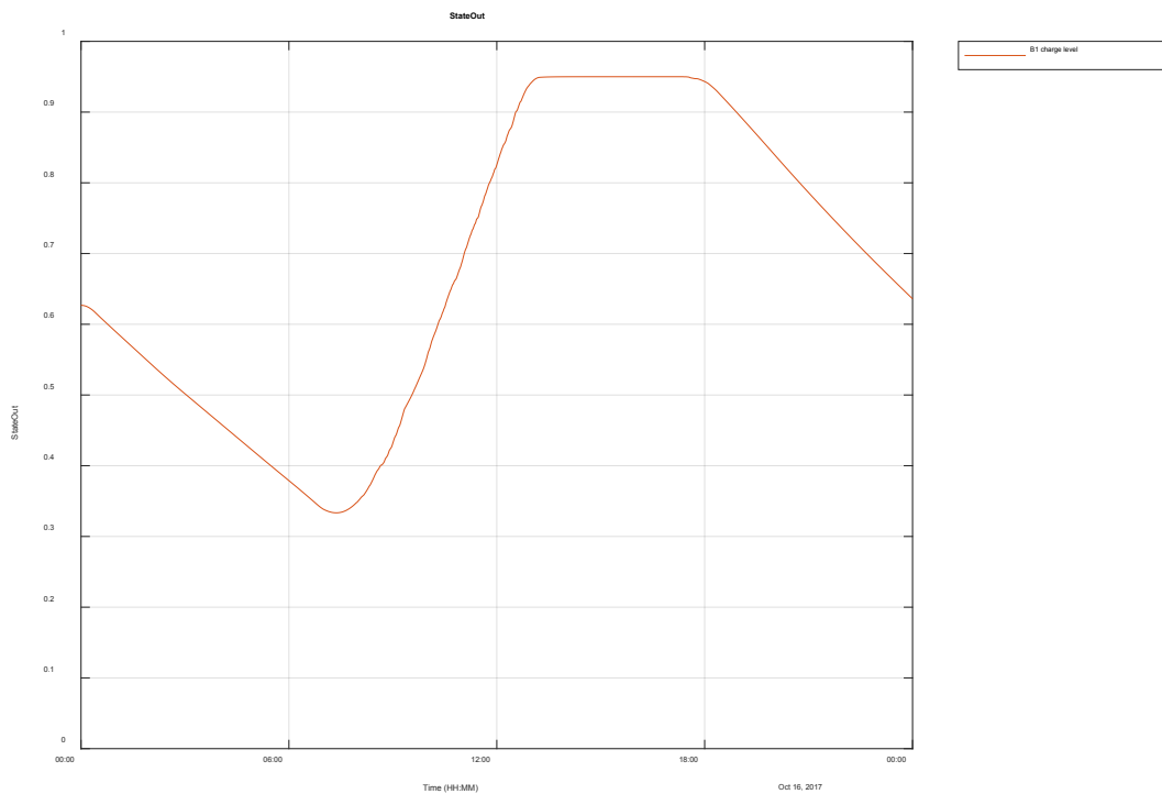
Figure 3-58 Simulated battery charge level for weekday when 2.5 MW / 13 MWh battery provides both primary frequency control and AGC with 4.3 MW of PV.
