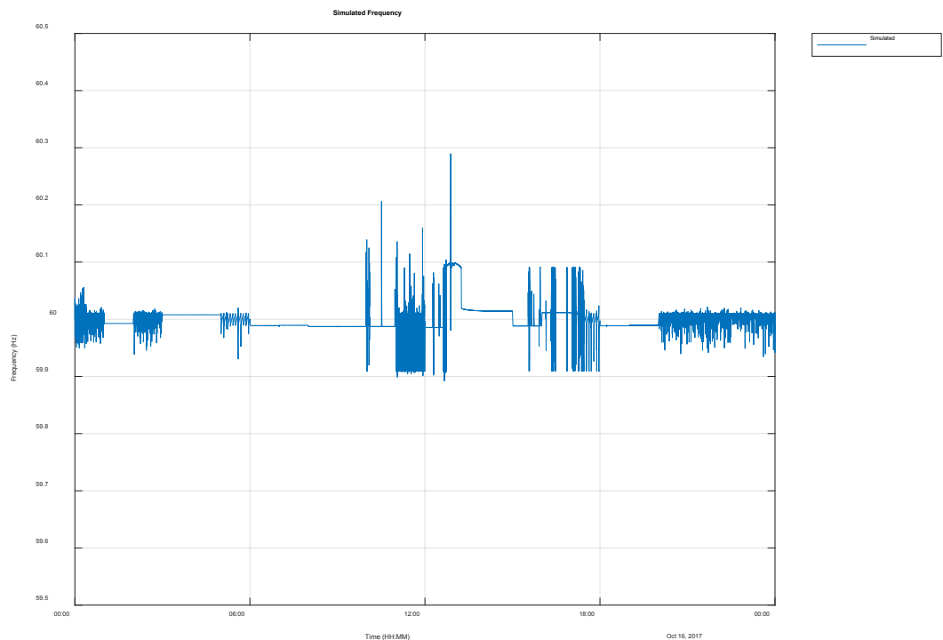
Figure 3-60 Simulated frequency for weekend when 2.5 MW / 13 MWh battery provides both primary frequency control and AGC with 4.3 MW of PV.
