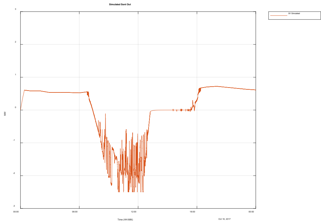
Figure 3-57 Simulated battery output for weekday when 2.5 MW / 13 MWh battery provides both primary frequency control and AGC with 4.3 MW of PV.
