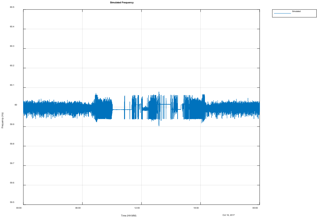
Figure 3-64 Case 20 - Simulated frequency on weekday with 1 MW PV and 0.5 MW battery on primary frequency control
