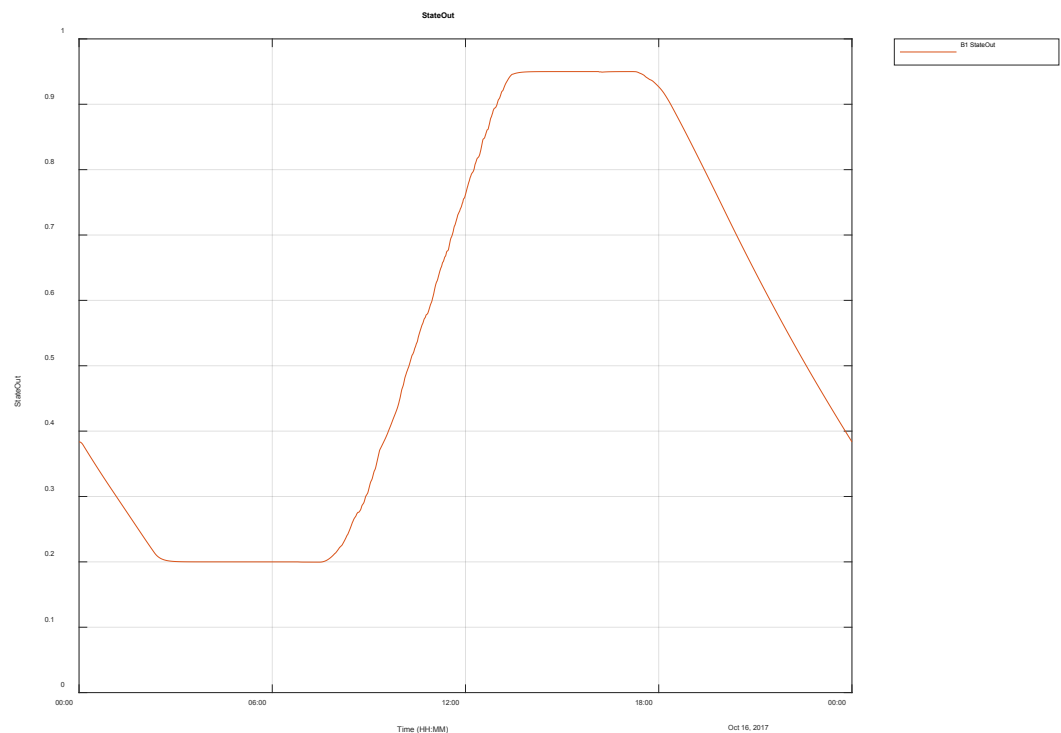
Figure 3-53 Simulated battery charge level for weekday when 1.25 MW / 5 MWh battery provides both primary frequency control and AGC with 2.3 MW of PV.
