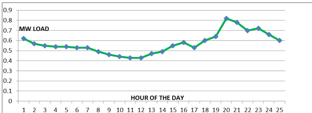
Figure 3-10 Typical weekend profile for Kosrae
