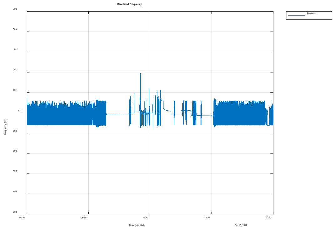
Figure 3-29 Simulated frequency for weekend when 1.25 MW / 5 MWh battery provides both primary frequency control and AGC with 2.3 MW of PV. All diesel units allowed to go off.
