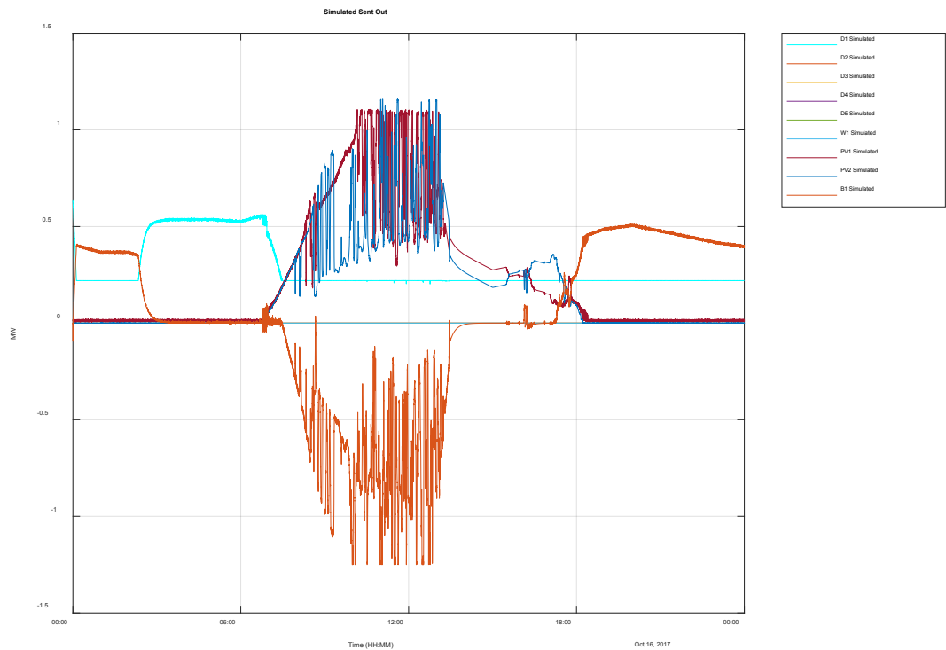
Figure 3-54 Simulated generator outputs for weekday when 1.25 MW / 5 MWh battery provides both primary frequency control and AGC with 2.3 MW of PV.
