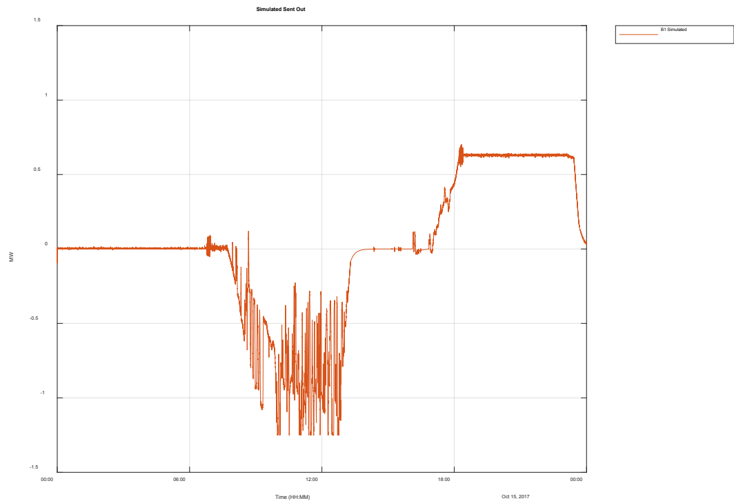
Figure 3-30 Simulated battery output for weekend when 1.25 MW / 5 MWh battery provides both primary frequency control and AGC with 2.3 MW of PV. All diesel units allowed to go off.
