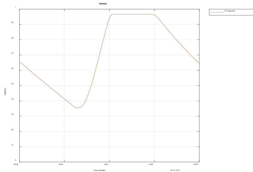
Figure 3-40 Case 12 - Simulated charge level on weekday with 4.3 MW PV and 2.5 MW / 13 MWh battery on AGC and all diesel units off.
