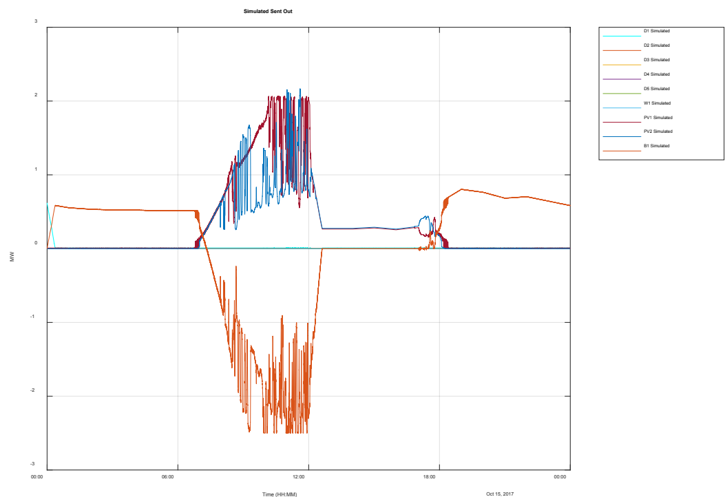
Figure 3-33 Simulated generator outputs for weekend when 2.5 MW / 13 MWh battery provides both primary frequency control and AGC with 4.3 MW of PV.
