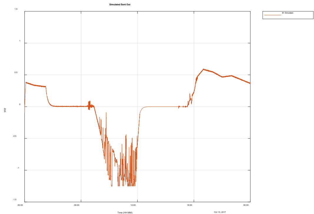
Figure 3-26 Simulated battery output for weekend when 1.25 MW / 5 MWh battery provides both primary frequency control and AGC with 2.3 MW of PV.
