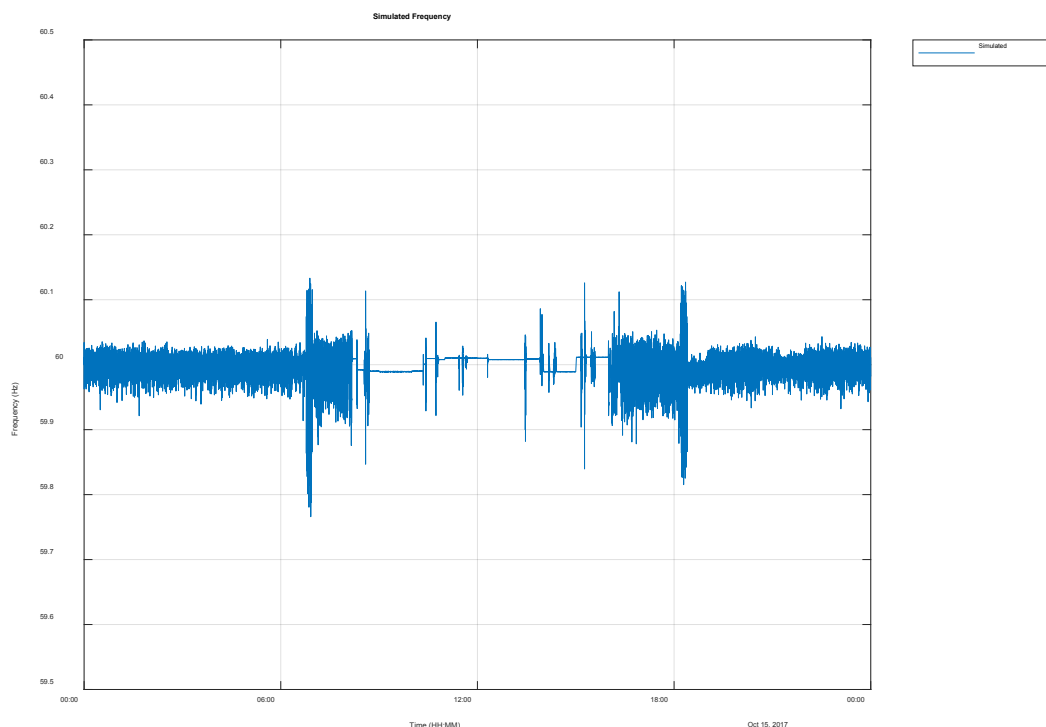
Figure 3-18 Simulated frequency on weekend with 1 MW PV
