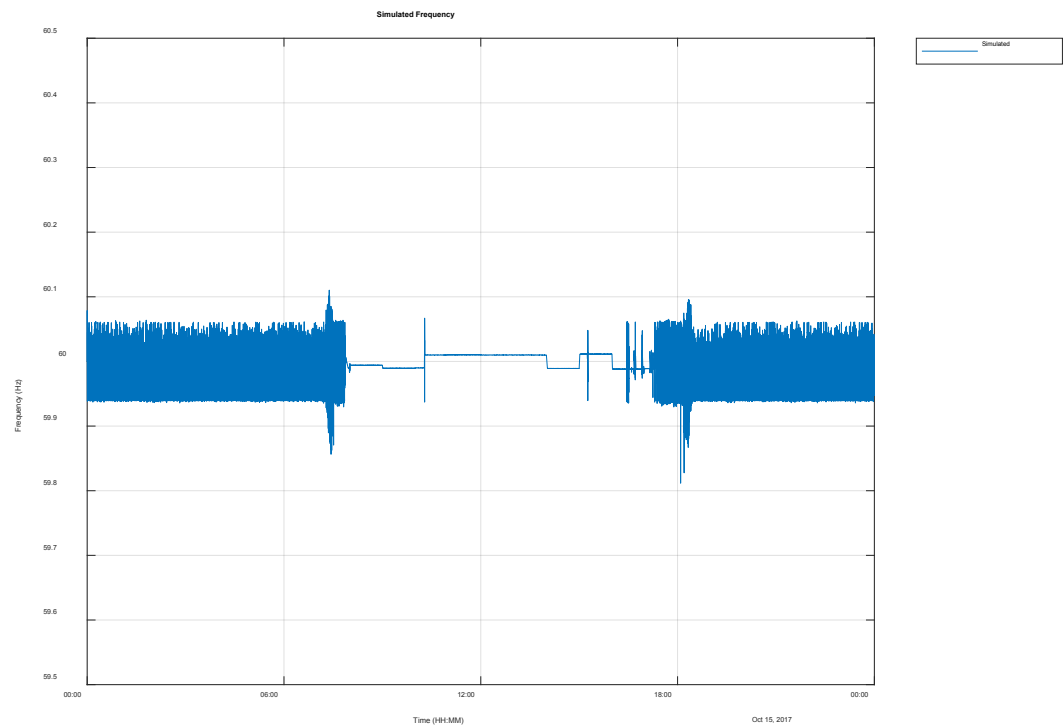
Figure 3-39 Case 9 - Simulated frequency on weekday with 2.3 MW PV and 0.5 MW battery on primary frequency control.
