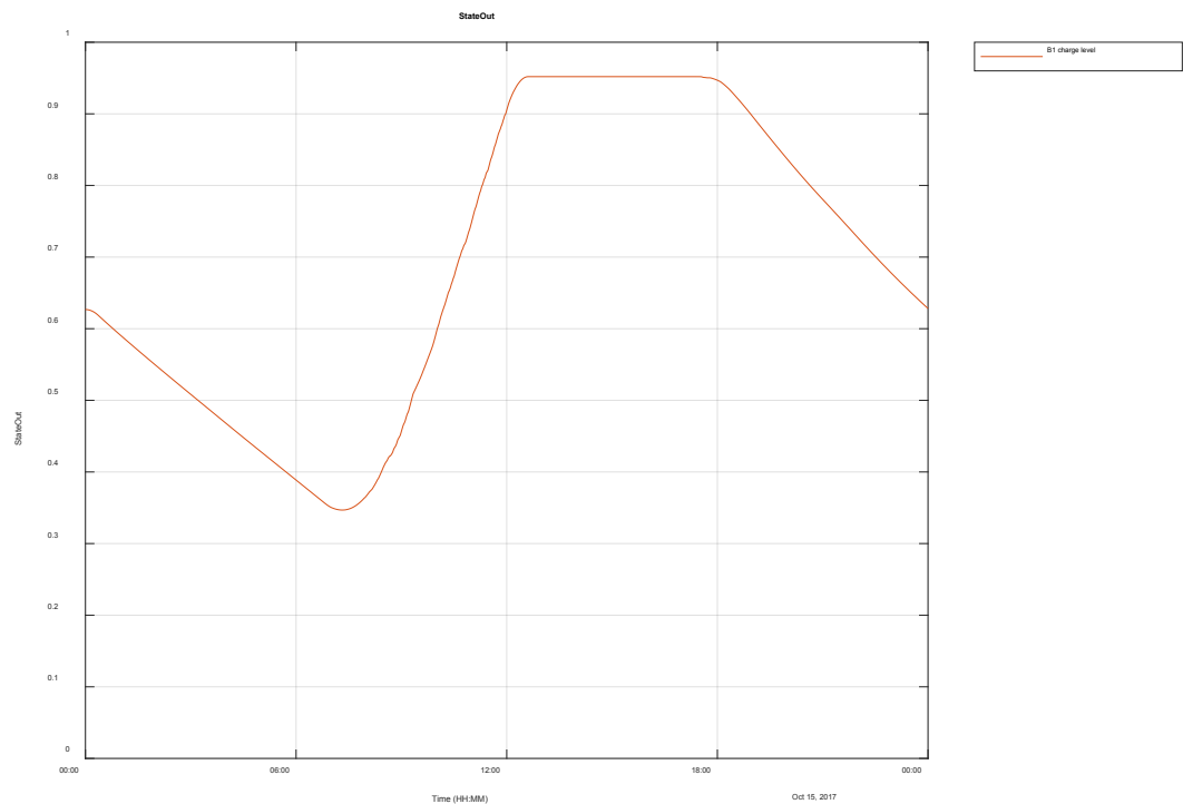
Figure 3-32 Simulated battery charge level for weekend when 2.5 MW / 13 MWh battery provides both primary frequency control and AGC with 4.3 MW of PV.
