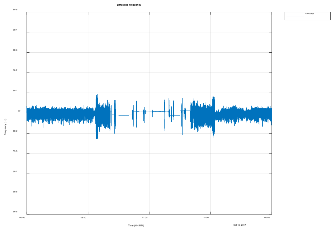
Figure 3-20 Simulated frequency for weekend with 1 MW of PV and 0.5 MW battery on primary frequency control
