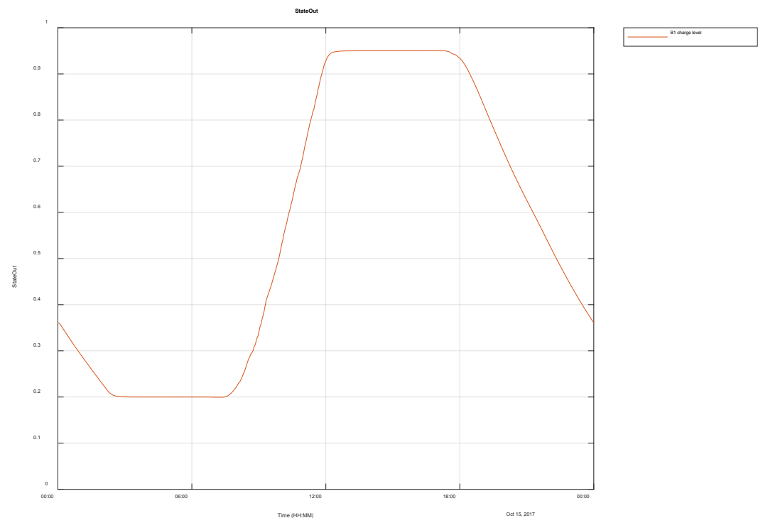
Figure 3-27 Simulated battery charge level for weekend when 1.25 MW / 5 MWh battery provides both primary frequency control and AGC with 2.3 MW of PV.
