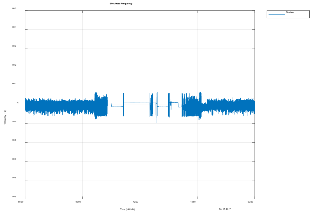
Figure 3-38 Case 8 - Simulated frequency on weekday with 1 MW PV and 0.5 MW battery on primary frequency control
