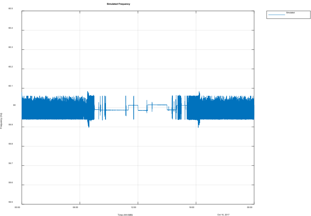
Figure 3-50 Simulated frequency for weekday with 2.3 MW of PV and 0.5 MW battery on primary frequency control
