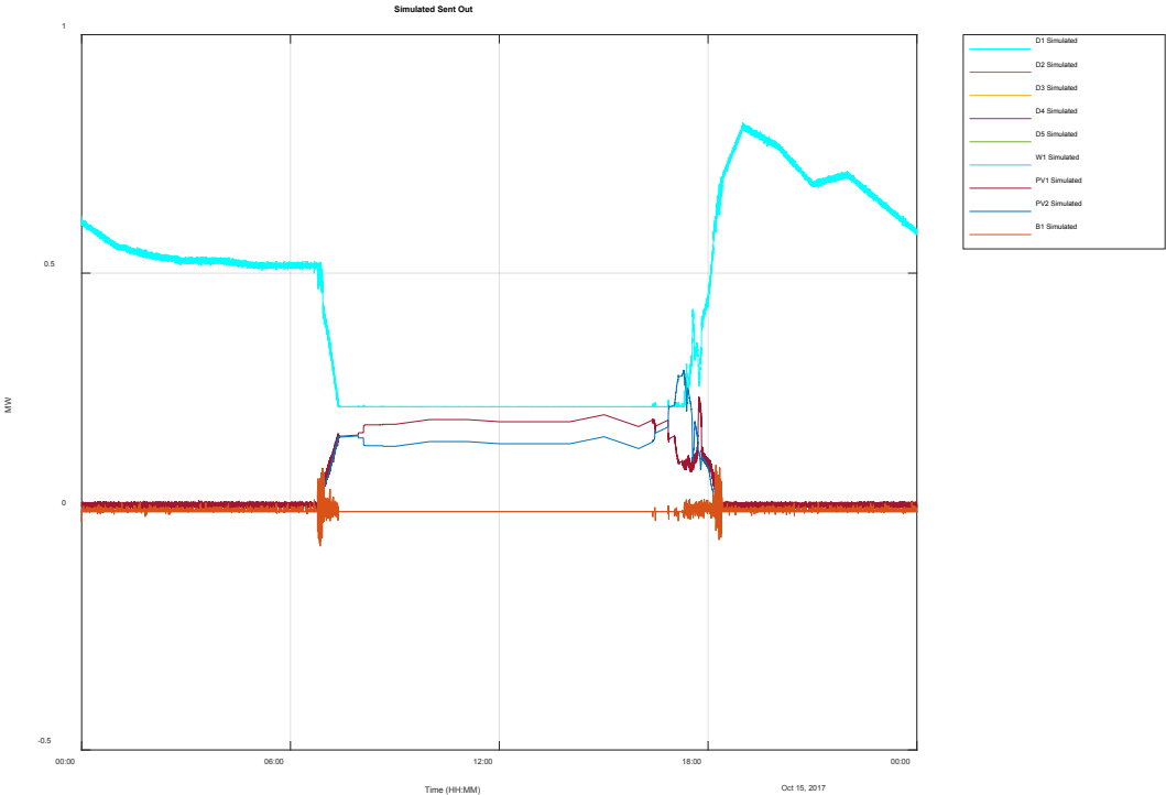
Figure 3-23 Simulated generation for weekend with 2.3 MW of PV and 0.5 MW battery on primary frequency control
