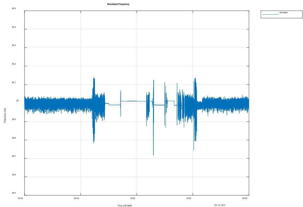
Figure 3-37 Case 7 - Simulated frequency on weekday with 1 MW PV
