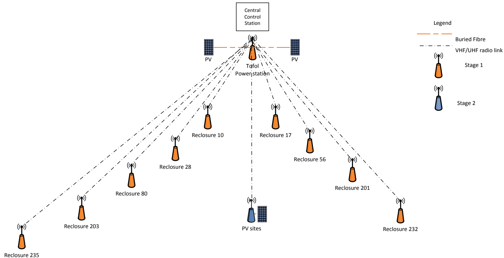
Figure 5-2: Concept communication network diagram for Kosrae network
