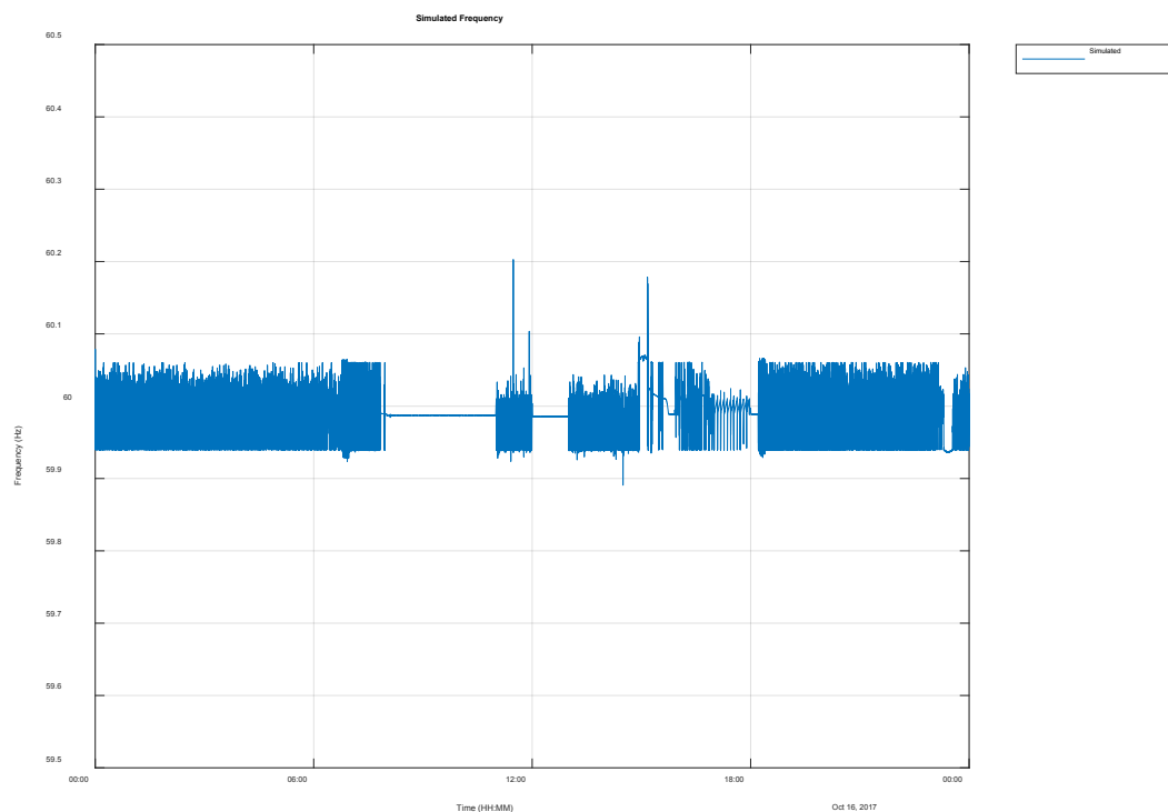
Figure 3-55 Simulated frequency for weekday when 1.25 MW / 5 MWh battery provides both primary frequency control and AGC with 2.3 MW of PV. All diesel units allowed to go off.
