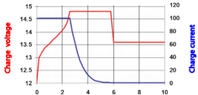
Fig. 3: Three step charge curve
