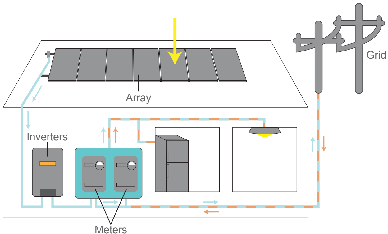
Figure 1: Grid connected PV systems
