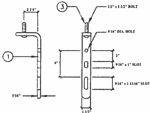
BRACKET DETAIL
