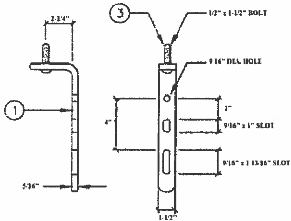
BRACKET DETAIL
