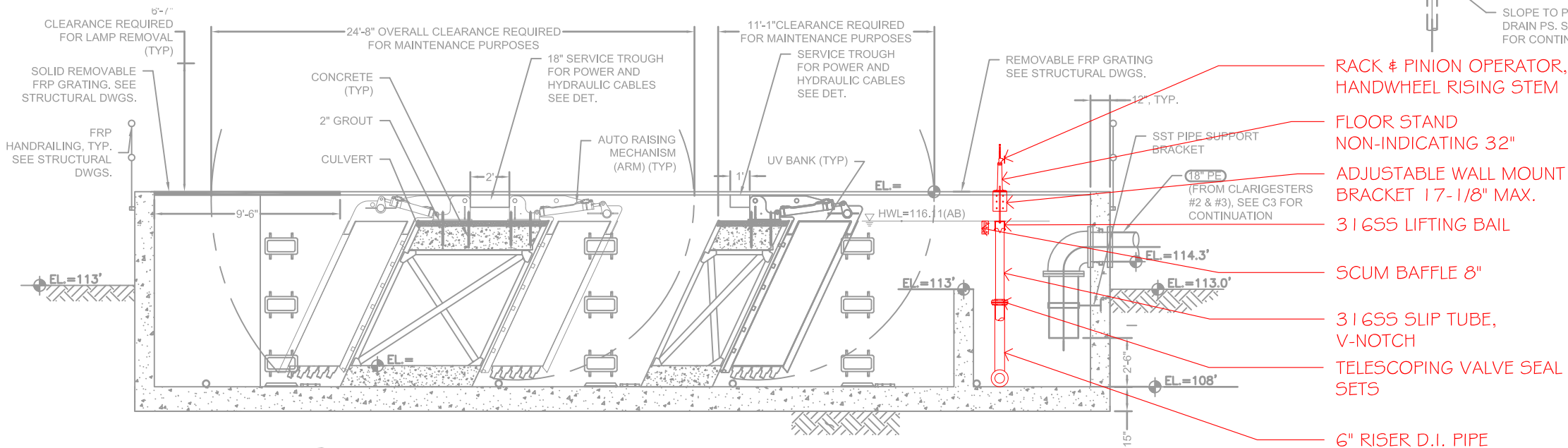
2 TAFUNA UV TANK LONG. SECTION Scale: NTS
