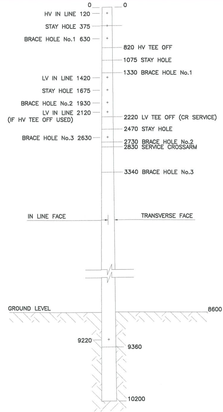
POLE TYPE 4 10.2m
