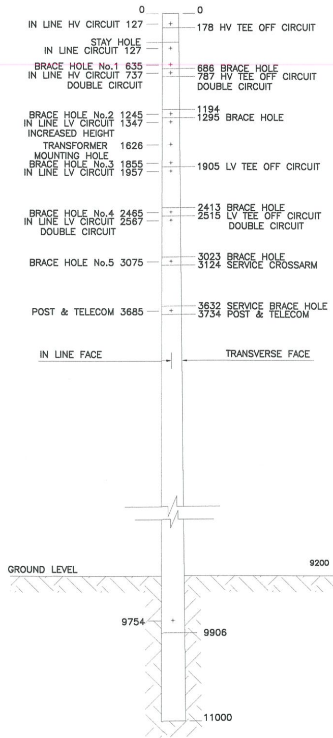
POLE TYPE 3 11m
